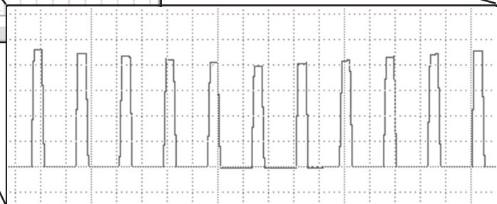
Inset showing the fully expanded PWM waveform.
