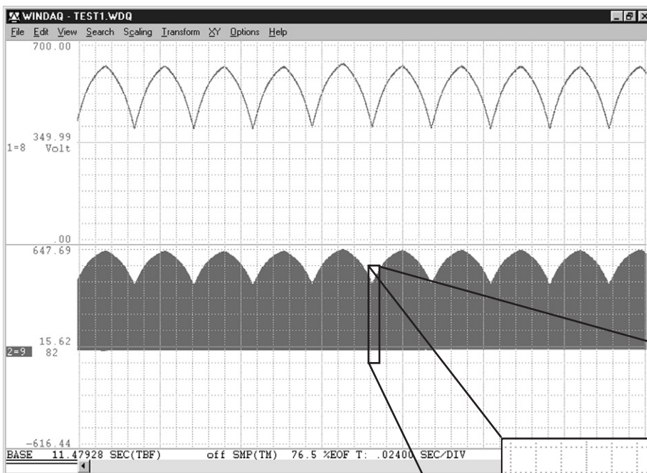
DC drive system waveforms acquired with a DI-730 and WINDAQ software. Shown compressed by a factor of 30, the top waveform is the sum of three-phase, full-wave rectified AC power. The bottom channel is the pulse width modulated waveform delivered to the DC motor for speed control.
