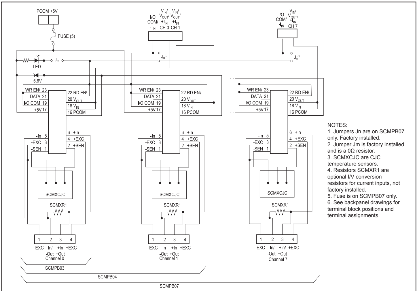
Figure 11: SCMPB03/SCMPB04/SCMPB07 Schematic
