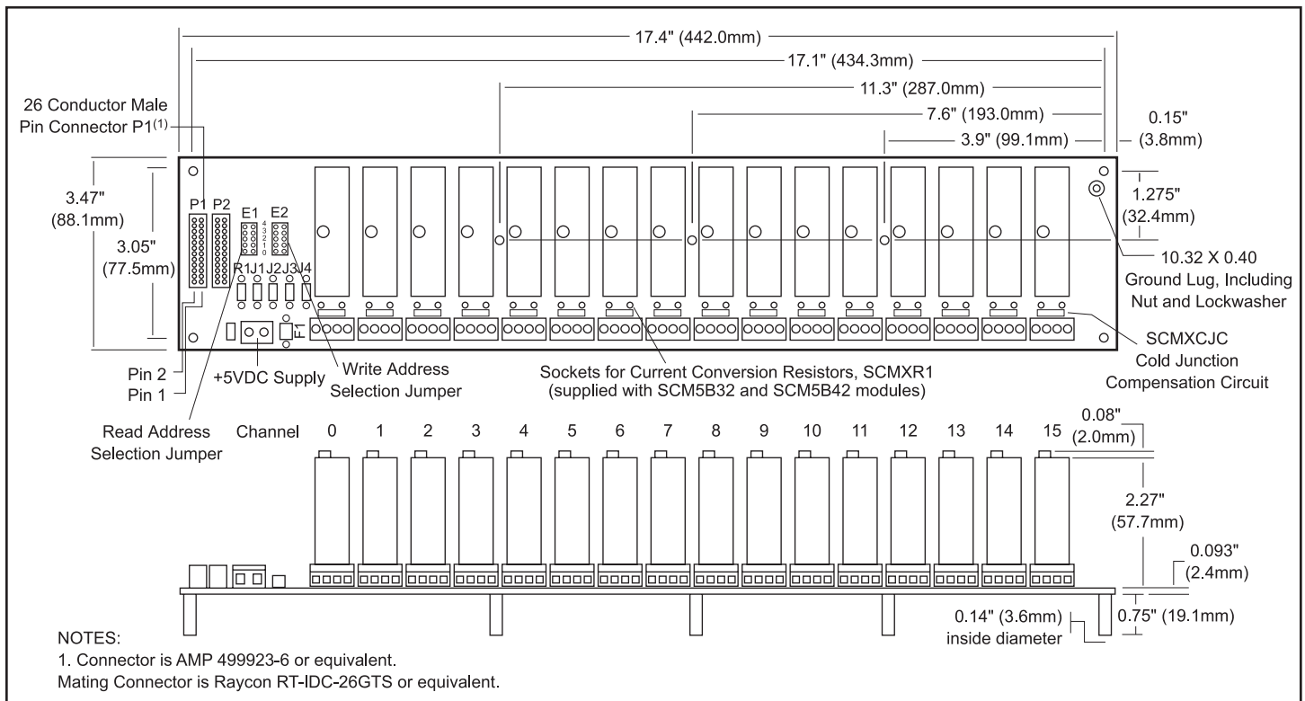
Figure 5: SCMPB02 Analog I/O Backpanel
