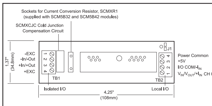
Figure 9: SCMPB03 Analog I/O Backpanel
