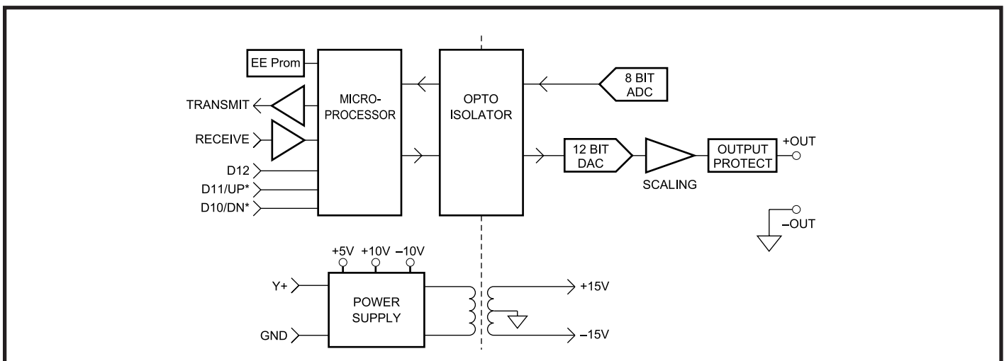
Figure 1: SCM9B-3000/4000 Block Diagram
