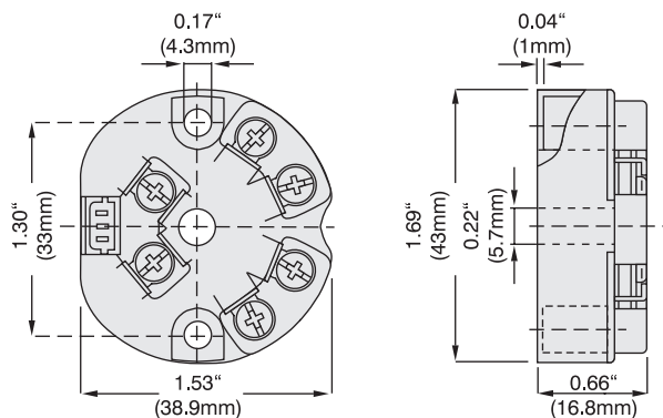
SCTP20-01 Input/Output Not Electrically Isolated
